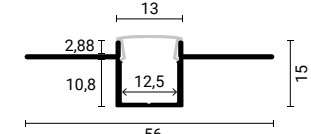
SKU 5162 Silver Body - White Cover (L=2m)
