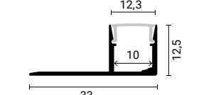
SKU 5111 Silver Body - White Cover (L=2m)
