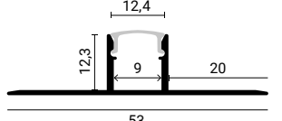
SKU 5112 Silver Body - White Cover (L=2m)
