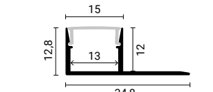
SKU 5144 Silver Body - White Cover (L=2m)
