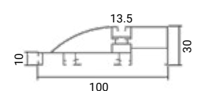
SKU 15122 Black Body- White Cover (L=2m)
